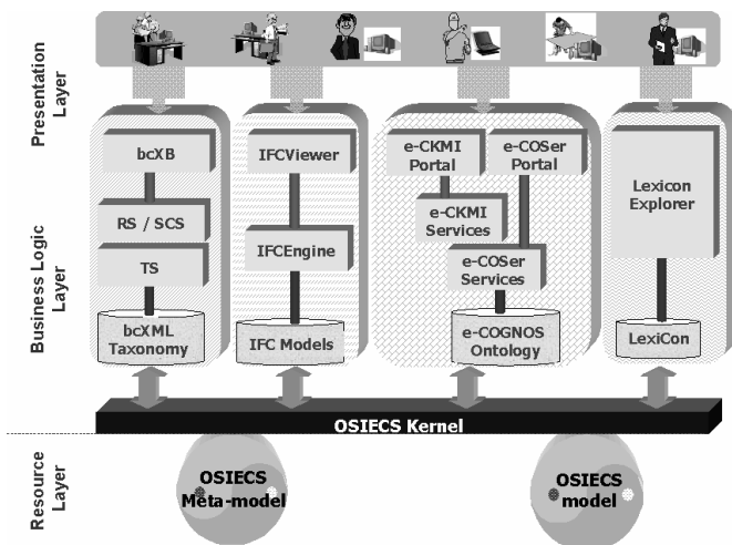
Figura 5. The ideal usage scenario for OSIECS components.
